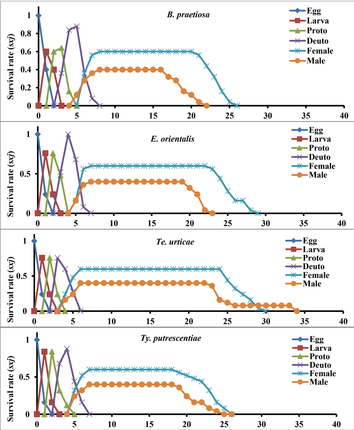
Figure 1. Age-stage specific survival rate ( s_{xj} ) of Neoseiulus californicus reared on four prey species at 27 \pm 1 °C.
