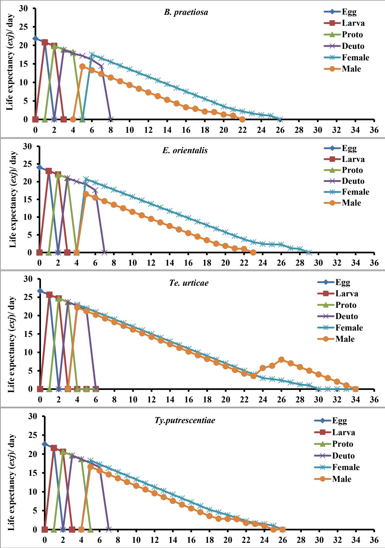
Figure 3. Age-stage life expectancy ( e_{xj} ) of Neoseiulus californicus reared on four prey species at 27 \pm 1^\circ\text{C} .
